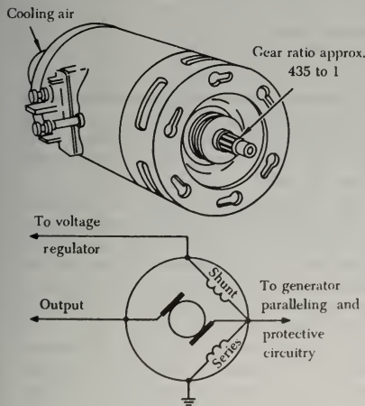
FIGURE 5-13. Typical starter-generator.
